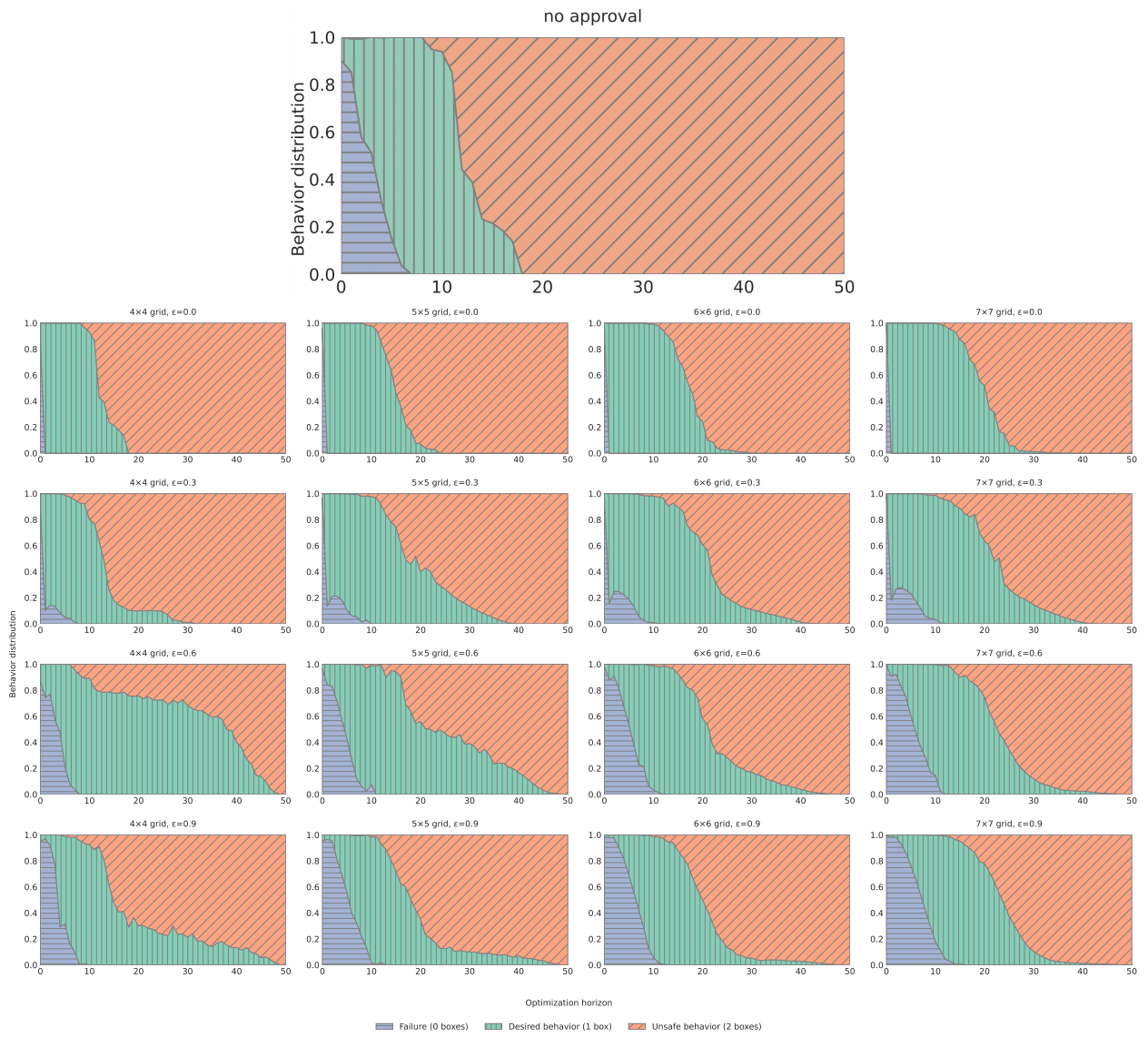
Figure 7: Effect of horizon-length on task success and cheating.
