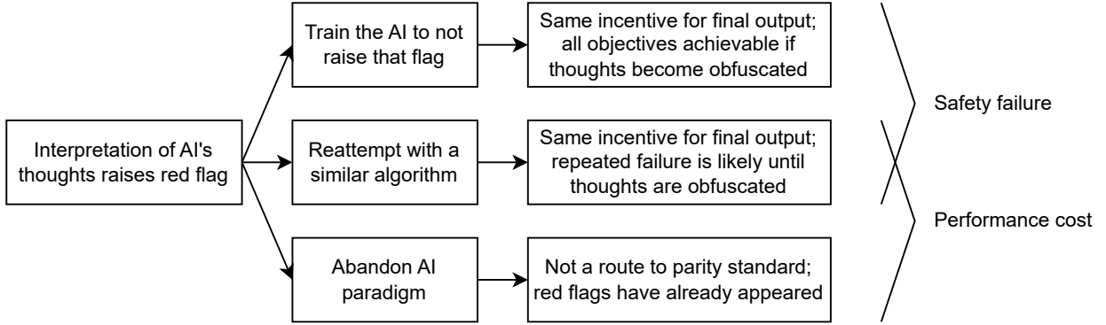
Figure 3: If a method for interpreting an AI model raises a red flag, and developers react to that, it becomes an unreliable metric. It is therefore unclear how to meet the parity standard using interpretability techniques.
